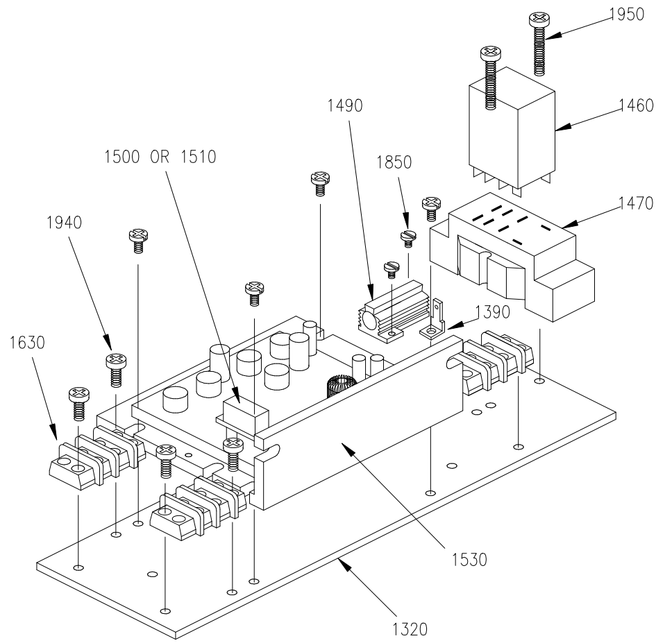
ELECTRICAL CHASSIS
